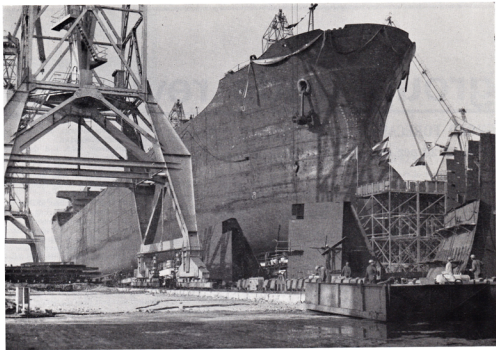
■ On the stocks just prior to her launching, the new B&C bulk carrier King Charles shows her massive, functional shape.
